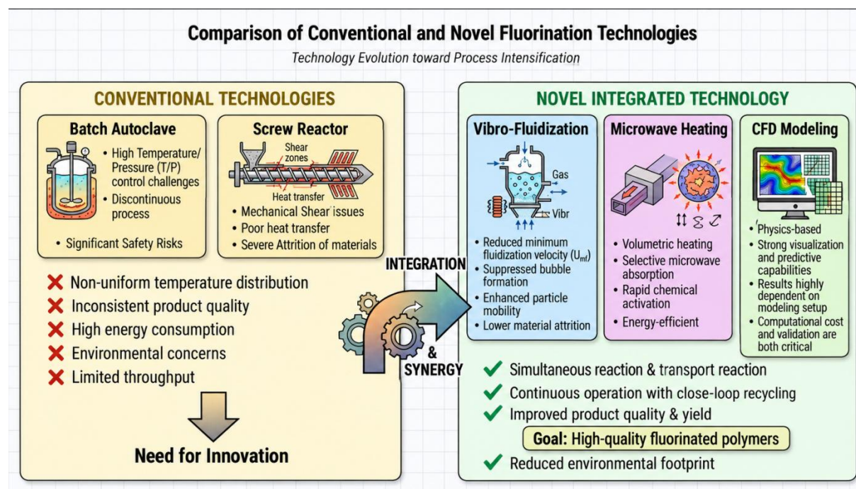
Figure 2. Comparison of conventional fluorination technologies (batch autoclave and screw reactor) and the proposed novel integrated technology.
