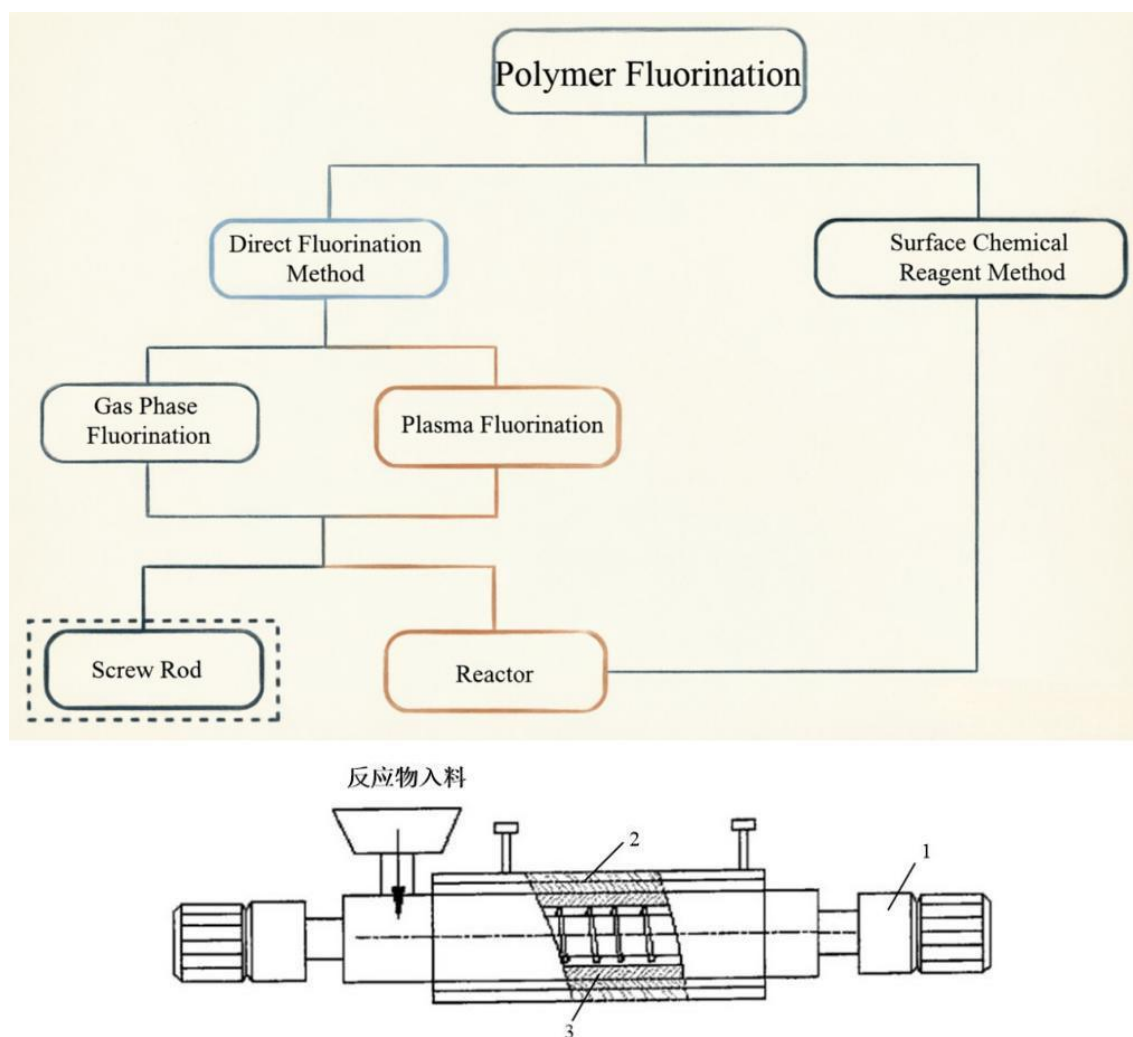
Figure 1. (a) Reactor for the production of fluorinated polymers; (b) Screw reactor (1—Motor; 2—High-temperature heating jacket; 3—Screw shaft).
