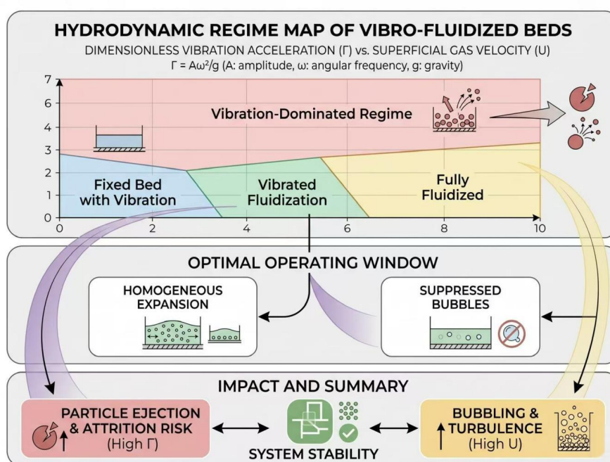
Figure 3. Hydrodynamic regime map of vibro-fluidized beds as a function of dimensionless vibration acceleration.
