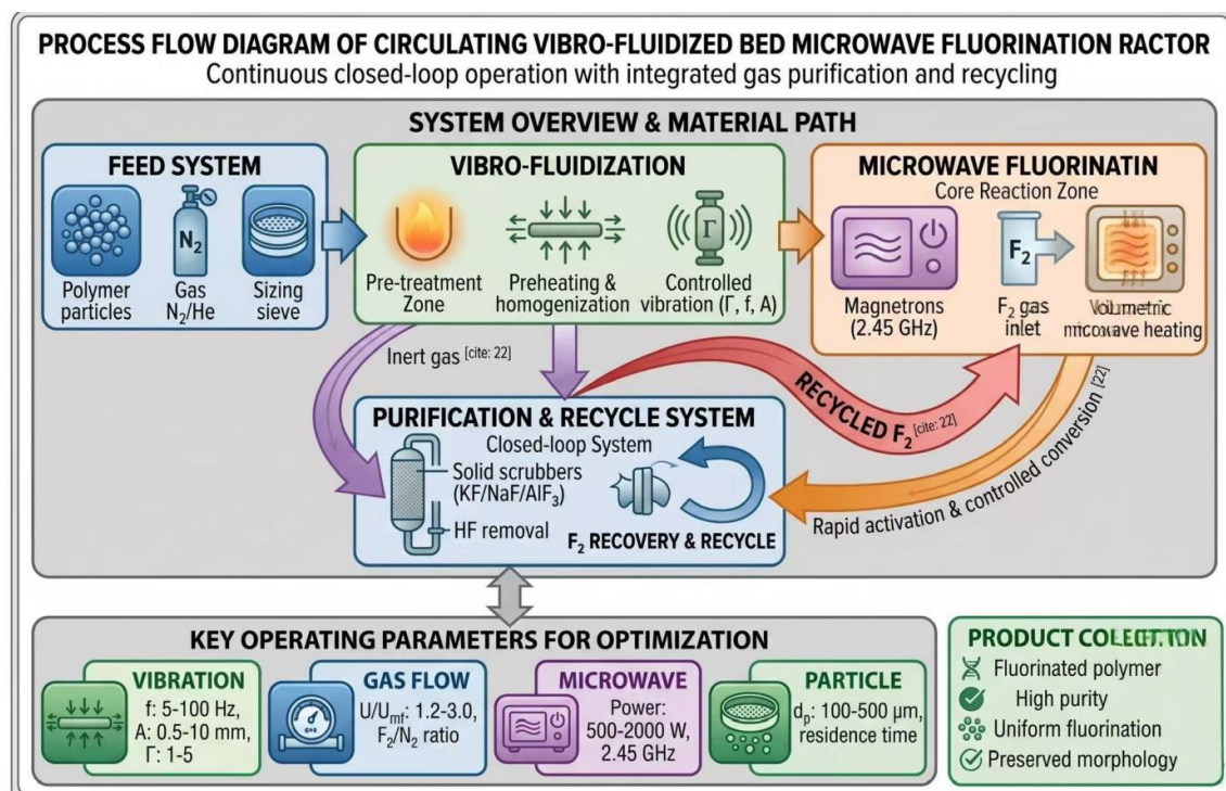
Figure 6. Process flow diagram of the circulating vibro-fluidized bed microwave fluorination reactor.
