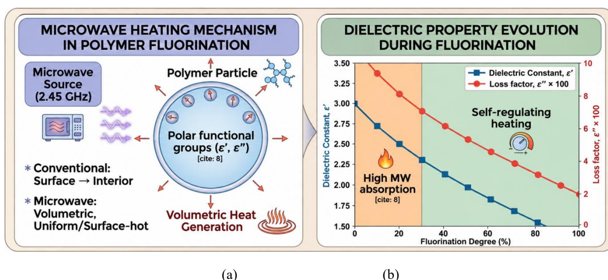
Figure 4. (a) Schematic illustration of microwave heating mechanism in polymer fluorination; (b) Evolution of dielectric properties ( \epsilon' and \epsilon'' ) as a function of fluorination degree.
