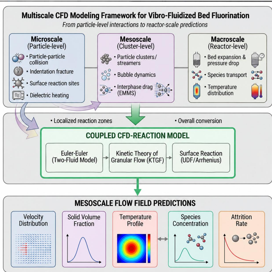
Figure 5. Multiscale CFD modeling framework for vibro-fluidized bed fluorination reactors.
